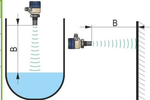
Use level in tank or a fix target e.g. the wall
